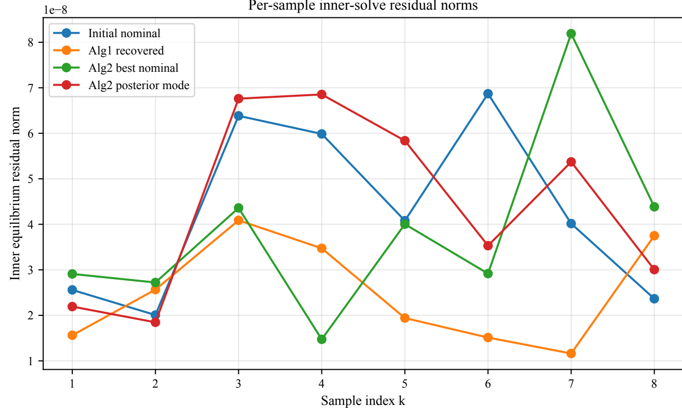
Per-sample inner-solve residual norms
